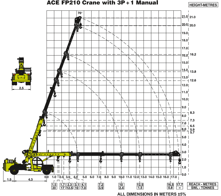
ACE FP210 Crane with 3P + 1 Manual
